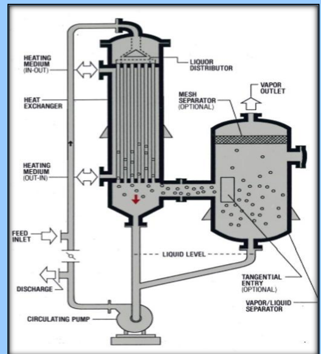
FALLING FILM EVAPORATION
