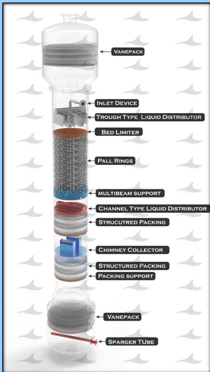
PACKED COLUMN
