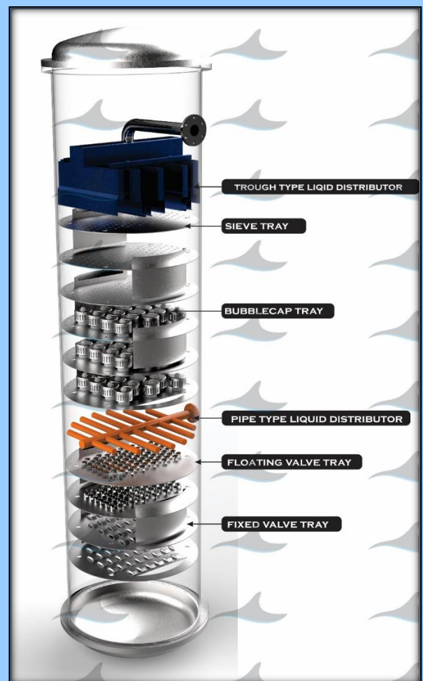
TRAY COLUMN
