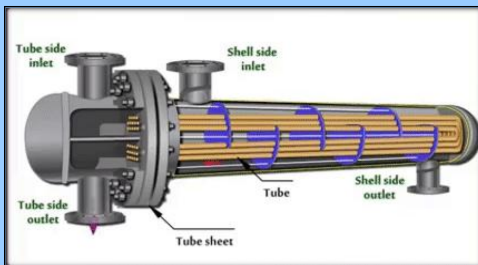
Shell and Tube Heat Exchanger
