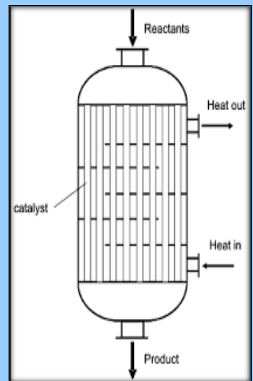
Tubular Reactor
