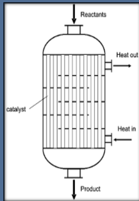
Tubular Reactor
