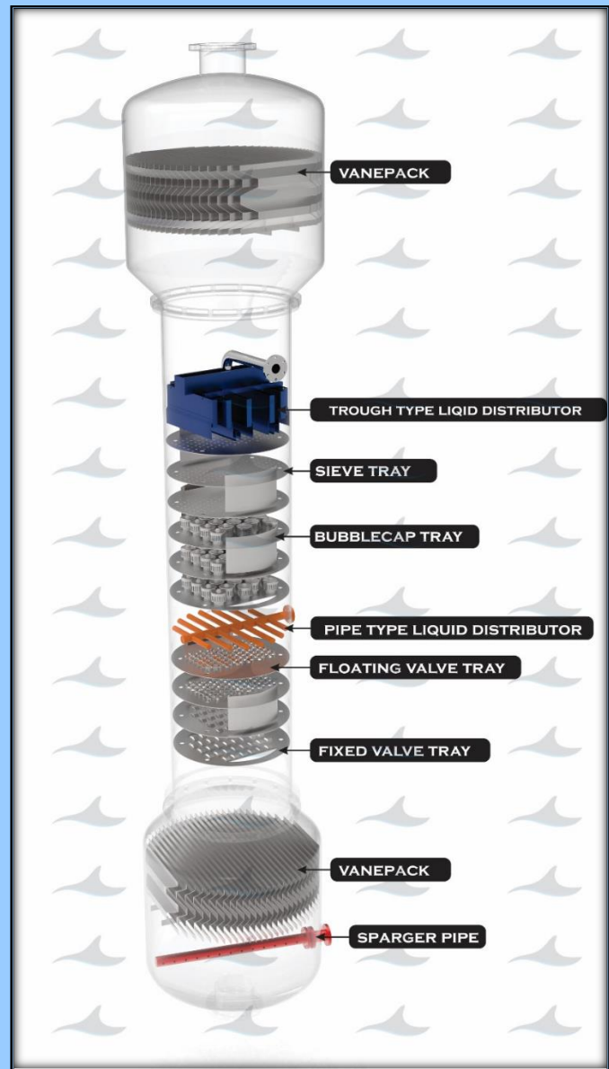
TRAY COLUMN
