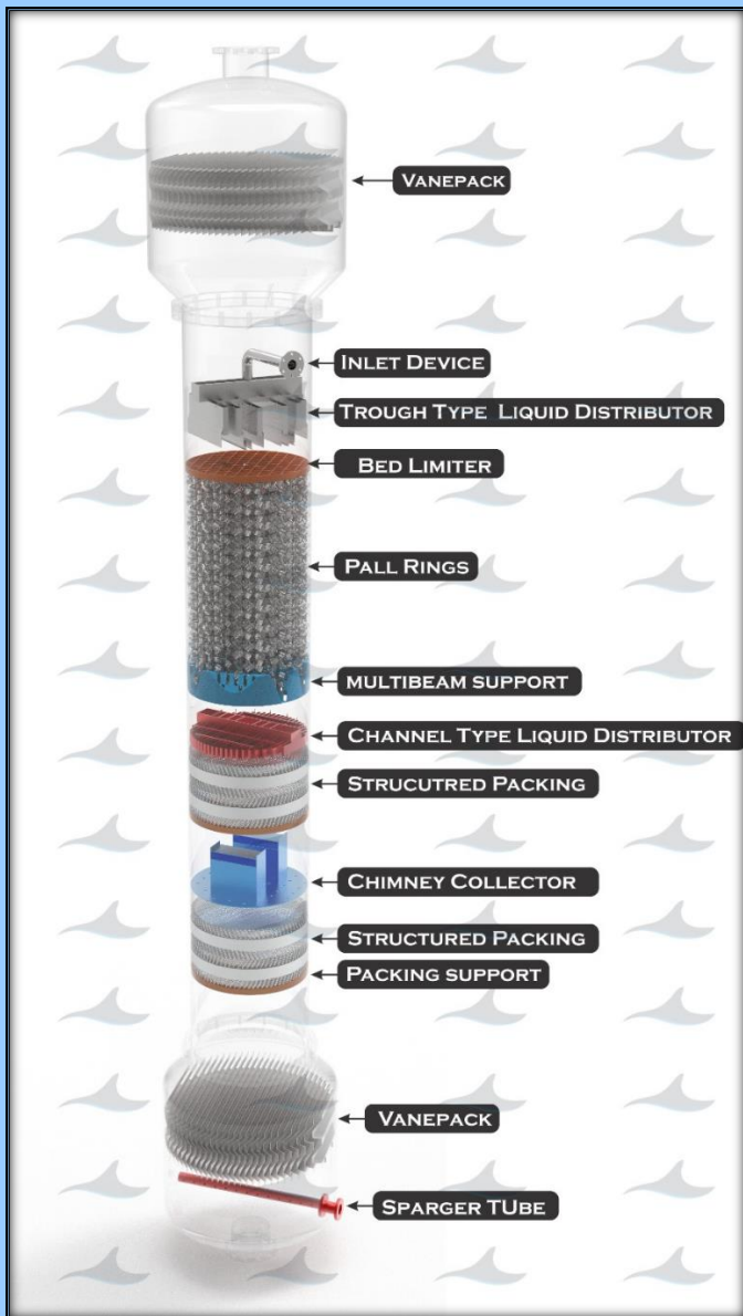
PACKED COLUMN
